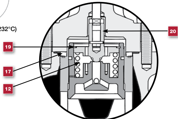
Pilot Balanced Construction Model 41405 Applications above 450°F (232°C) to 1050°F (566°C) Sizes 6" to 18" shown
