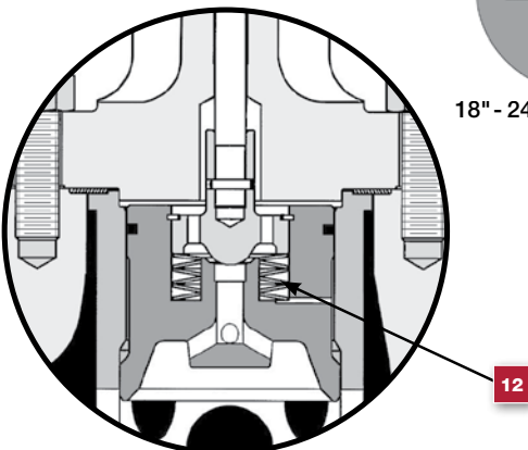
Pilot Balanced Construction Model 41405 Sizes 2" to 4" shown
