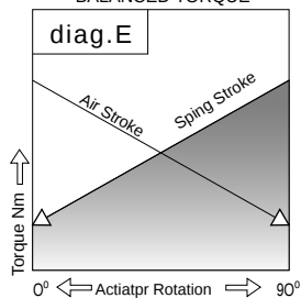
BALANCED TORQUE
