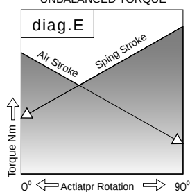
UNBALANCED TORQUE
